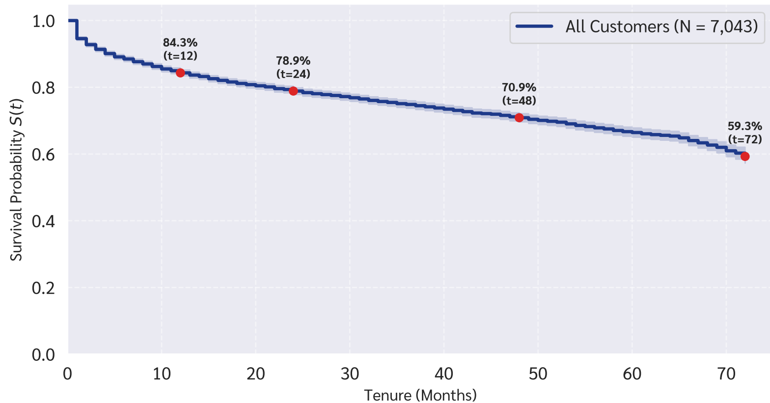
Overall Customer Kaplan-Meier Survival Curve \hat{S}(t)
